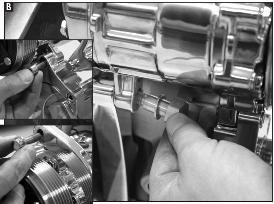
Figure 10: Install A/C Compressor
